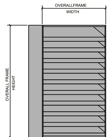
AL-300 LOUVRE FRAME
